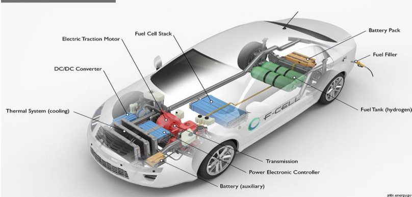
Hydrogen Fuel Cell Vehicle
